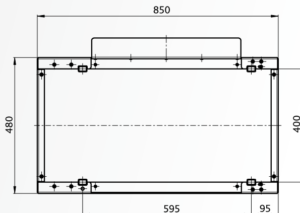
Ground plan of fastening on the floor
